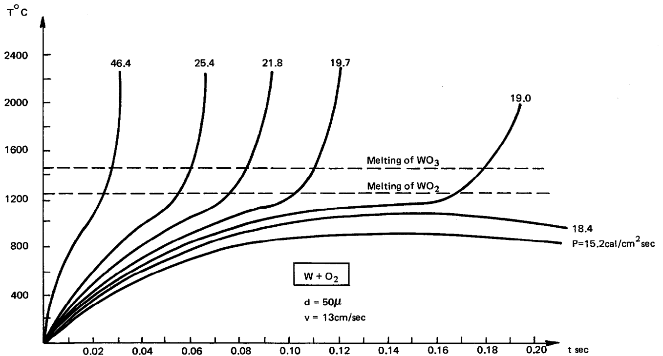
Fig 1 Thermogram of Tungsten Ignition in Oxygen
